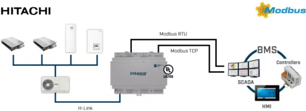
Integration example: when using the gateway to integrate mixed unit types like VRF and Air-to-water systems.
