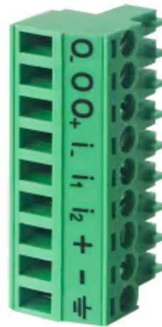
9-pole power and DI/DO connector for Ewon Cosy+ and Ewon Flexy
