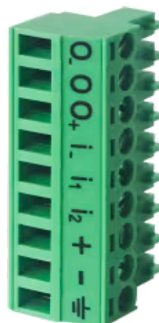
9-pole power and DI/DO connector for Ewon Cosy+ and Flexy devices
